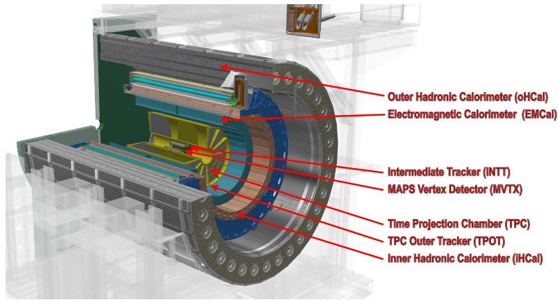
Figure 1: The sPHENIX Detector, with major detector components identified. Beginning from the collision point, particles pass through the tracking detectors (MVTX, INTT, and TPC), then electromagnetic, and finally, hadronic calorimeters. Between the inner and outer hadronic calorimeters is the coil and cryostat of the 1.4 T superconducting magnet. The TPOT detector is directly outside the TPC outer radius, covering \sim 90^\circ in \phi . Forward components, MBDs and EPD, are not shown.
