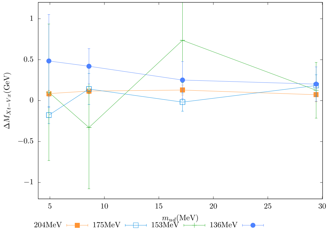
SU(2)_{CS} Symmetry Plot : Xt-Vx Screening Mass Difference
