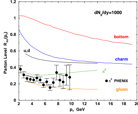
Figure 2: Parton-level nuclear modification factor R_{AA} in central Au+Au collisions, due to gluon bremsstrahlung in the DVGL framework, for various parton species. Figure is from [27].
