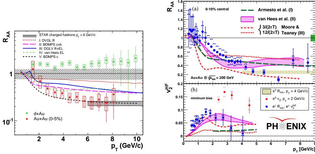
Figure 5: Nuclear modification factor R_{AA} for non-photonic electrons. Figures from [41, 43].
