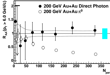
Figure 3: Nuclear modification factor R_{AA} for photons and \pi^0 as a function of N_{part} in Au+Au collisions at \sqrt{s_{NN}} = 200 \text{ GeV} from PHENIX. Figure is from [28].
