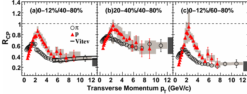
Figure 4: Binary-scaled ratio of central to peripheral spectra R_{CP} for pions and protons in \sqrt{s_{NN}} = 200 GeV Au+Au collisions from STAR. Point-to-point systematic uncertainties are shown as shaded boxes around the data points. Dark shaded bands show the normalization systematic uncertainty in the number of binary collisions N_{bin} . “Vitev” is a calculation for pions including energy loss from gluon bremsstrahlung [31]. Figure is from [32].
