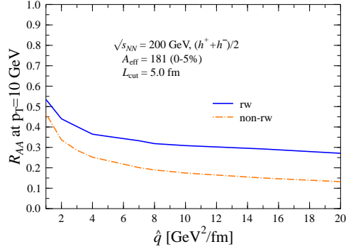
Figure 1: Predicted suppression factor R_{AA} vs \hat{q} , a measure of the color charge density of the medium. “rw” and “non-rw” refer to two different methods of taking into account energy conservation. Figure is from [14].
