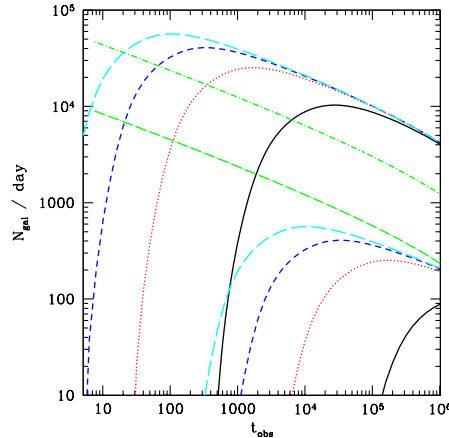
Figure 1: Predicted number of galaxies for a day of observing as a function of observation time per pointing. The straight green curves indicate FAST with 100 beams (upper, dotted-short-dash) and 19 beams (lower, dotted-long-dash) respectively. The upper sloped curves correspond to the 10% SKA with varying resolutions (in arcsec); 24 (cyan, large-dash), 18 (blue, short-dash), 12 (red, dot) and 6 (black, solid). The lower curves are for the case of the 1% SKA with the lines equating to the same resolutions as before.
