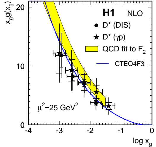
Figure 4: Gluon distribution.
