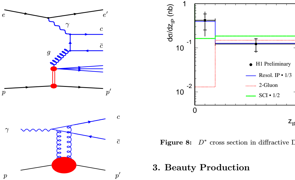
Figure 7: Diagrams of diffractive D^* production: “resolved Pomeron” (upper) and “2 gluon” model.
