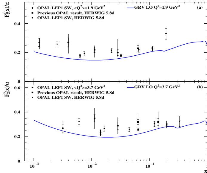
Figure 1: Photon structure function measured at the lowest x attainable at LEP. The inner error bars show the statistical error, while the outer error bars, where shown, correspond to the total error.
