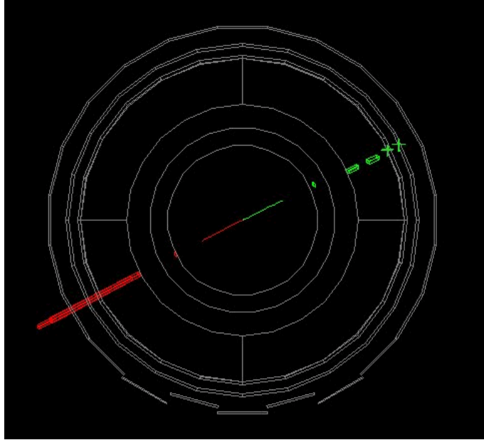
Figure 2: The production of a Z^0 particle that decays into a pair of tau leptons, which decay into an electron and a muon (plus unseen neutrinos), respectively.
