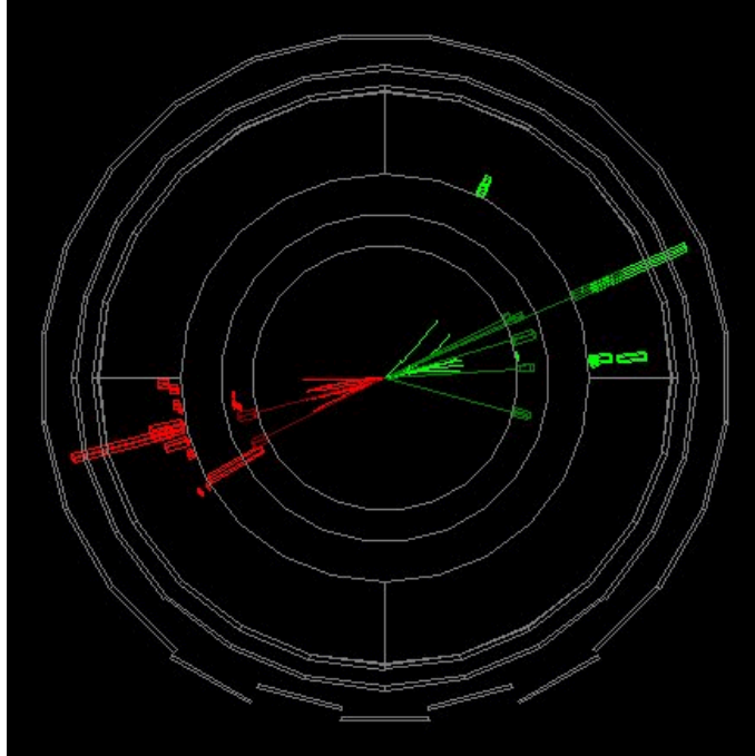
Figure 1: The production of a Z^0 particle that decays into a pair of quarks (a quark and an antiquark).
