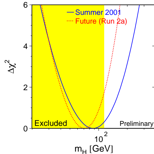
Figure 17: Typical \Delta\chi^2 curve obtained with m_W and m_{\text{top}} measurements of 20 MeV and 3 GeV precision, respectively (dashed) and compared to the current fit result central value (solid).
