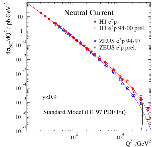
Figure 9: Neutral-current differential cross-sections measured at HERA[27].
