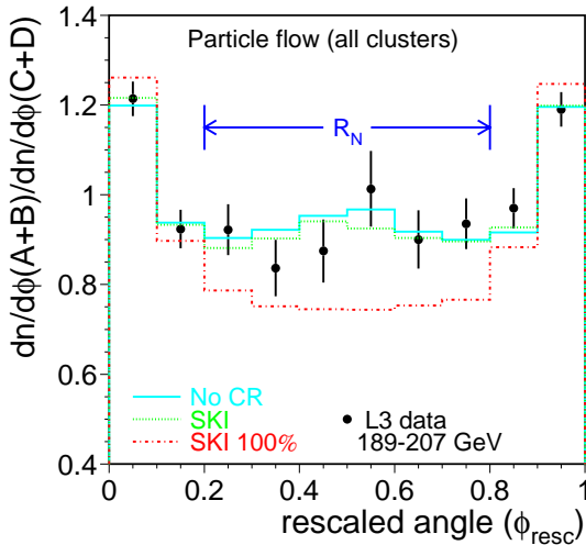
Figure 11: Particle flow ratio for particles between jets coming from the same W relative to those between jets from different W ’s[35]. Data are compared to models with no colour reconnection, and to the SKI model[36].
