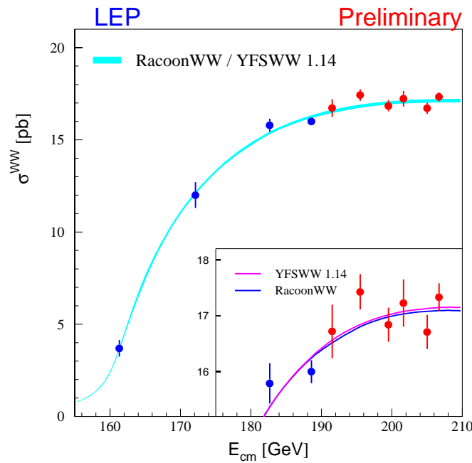
Figure 10: LEP averaged W-pair production cross-section measurements[29].
