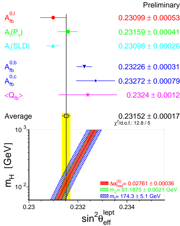
Figure 4: Comparison of asymmetry measurements interpreted simply as measurements of \sin^2 \theta_{\text{eff}}^{\text{lept}} .
