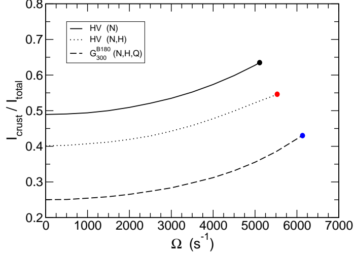
Figure 9: Moment of inertia of several sample neutron stars.
