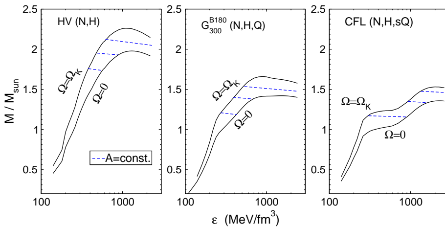
Figure 7: Mass–central energy relations for the sample equations of state introduced in Sect. 2.
