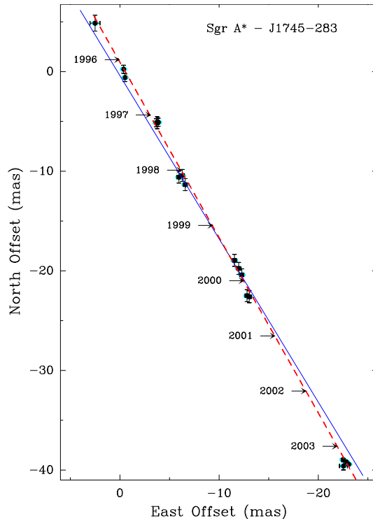
Figure 2: Apparent motion of Sgr A* relative to a background quasar. The blue line indicates the orientation of the Galactic plane and the dashed line is the variance-weighted best-fit proper motion. Taken from [18].
