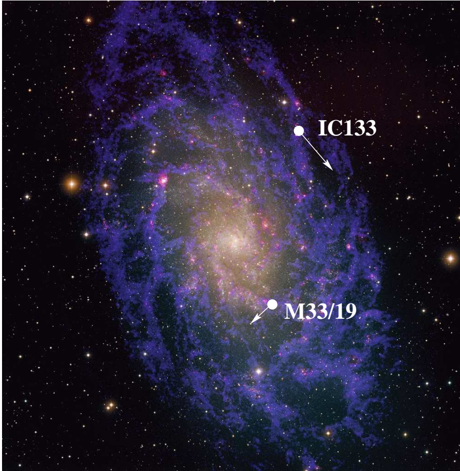
Figure 3: Position of two regions of maser activity in M33. Also shown are predicted motions due to rotation of the HI disk (shown in blue). The optical image of M33 was provided by Travis Rector (NRAO/AUI/NSF and NOAO/AURA/NSF), and the HI image by David Thilker (NRAO/AUI/NSF) and Robert Braun (ASTRON). Taken from [22].
