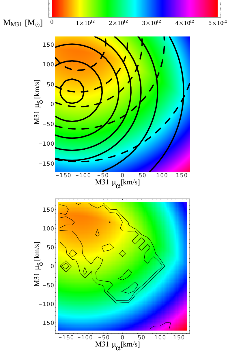
Figure 8: Top: Lower limit on the mass of M31 for different tangential motions of M31 assuming that M33 (dashed) or IC 10 (solid) are bound to M31. The lower limits are (4, 5, 7.5, 10, 15, 25) \times 10^{11} M_\odot for M33, and (0.7, 1, 2.5, 5, 7.5, 10, 15, 25) \times 10^{11} M_\odot for IC 10, rising from inside. The colour scale indicates the maximum of both values. Bottom: The colour scale is the same as above and gives the lower limit on the mass of M31. The contours show ranges of proper motions that would have lead to a large amount of stars stripped from the disk of M33 through interactions with M31 or the Milky Way in the past. The contours delineate 20% and 50% of the total number of stars stripped [32]. These regions can be excluded, since the stellar disk of M33 shows no signs of such interactions. Taken from [28].
