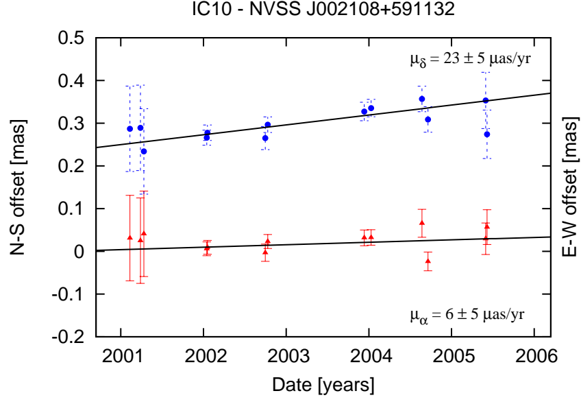
Figure 6: The position of the maser in IC 10 relative to a continuum background source in East-West (red triangles) and North-South (blue circles). The lines show a variance-weighted linear fit to the data points. Taken from [28].
