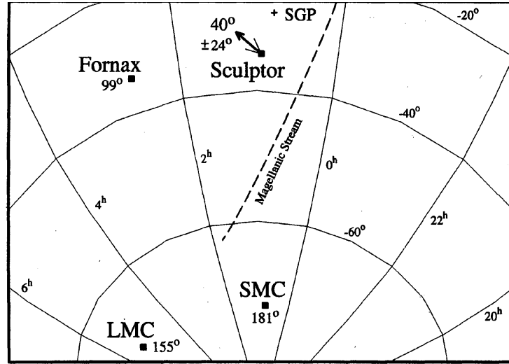
Figure 1: The proper motion of the Sculptor Dwarf Spheroidal Galaxy. Taken from [6].
