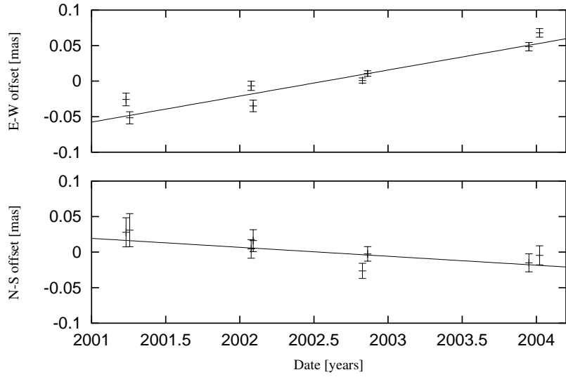
Figure 4: Average positions of the maser in M33/19 in East-West (upper) and North-South (lower) relative to the reference source. Taken from [22].
