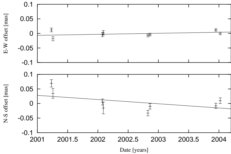
Figure 5: Average positions of the maser in IC 133 in East-West (upper) and North-South (lower) relative to the reference source. Taken from [22].
