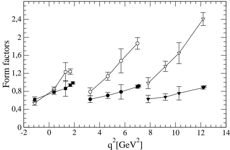
Figure 2: Form factors for semileptonic decays for various heavy quark masses. The light and spectator quark hopping parameters are fixed to the \kappa value 0.13498. Filled symbols denote F_0 , open symbols F_+ . Squares correspond to \kappa_h = 0.129 ( M_h = 2.1 GeV), circles to \kappa_h = 0.121 ( M_h = 3.4 GeV), and triangles to \kappa_h = 0.115 ( M_h = 4.2 GeV).
