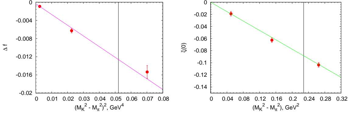
Figure 3: Interpolation of \Delta f (Left) and \xi(0) (Right) to physical meson masses indicated by the vertical lines.
