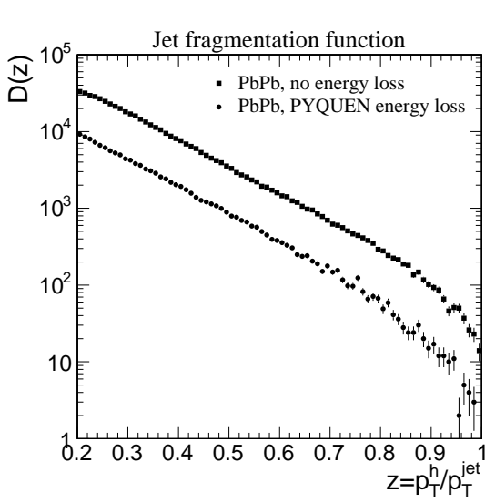
Figure 7: Jet fragmentation function for leading hadrons ( E_T^{\text{jet}} > 100 GeV) in central PbPb collisions without (squares) and with (circles) partonic energy loss. The number of histogram entries and statistical errors correspond to the estimated jet rate for one month of LHC running.
