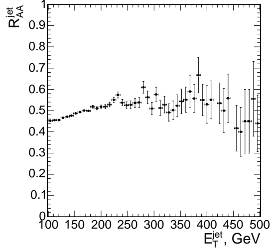
Figure 6: The nuclear modification factor, R_{AA}^{\text{jet}}(p_T) , for jets of cone size R = 0.5 in central PbPb collisions. The number of histogram entries and statistical errors correspond to the estimated event rate for one month of LHC running.
