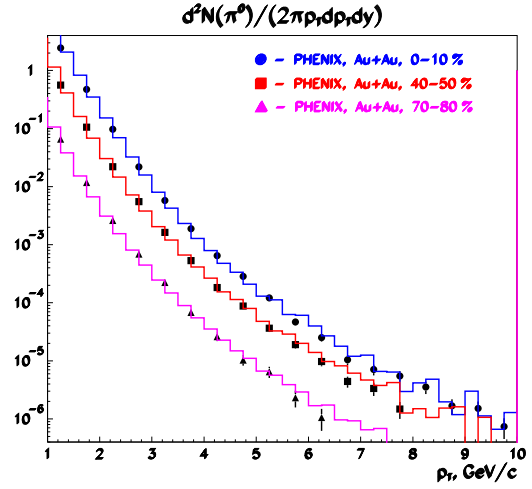
Figure 2: The transverse momentum distribution of neutral pions in AuAu collisions for three centrality sets. The points are PHENIX data, histograms are the model calculations.
