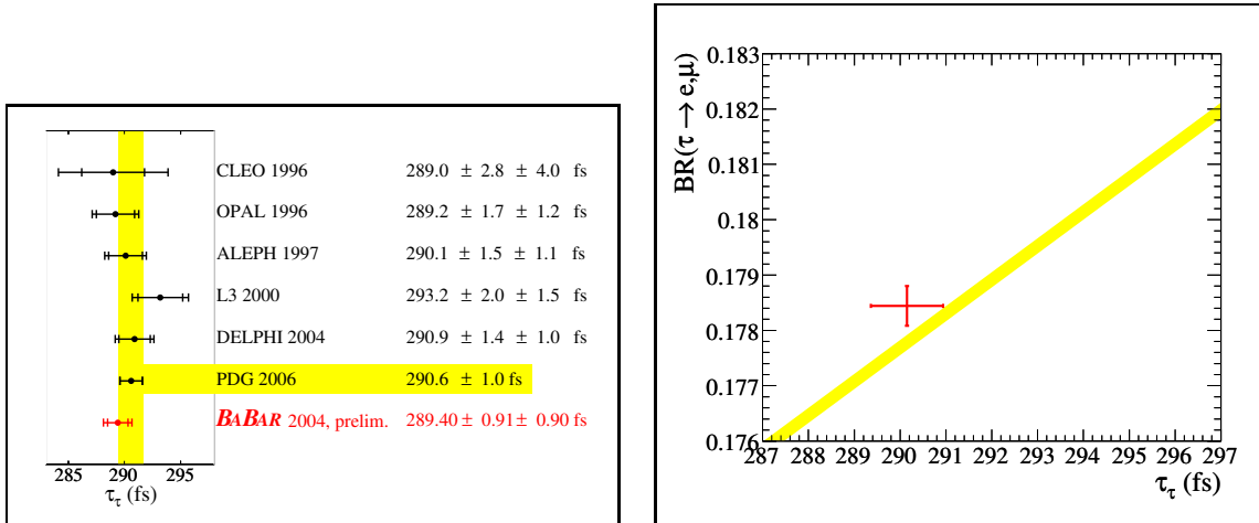
Figure 2: Selected tau lifetime measurements (left) and check of the Standard model (SM) prediction of universal leptonic couplings to the W (right) combining the present tau lifetime world average with the BABAR preliminary result. The thickness of the oblique line represents the uncertainty of the SM constraint, and is dominated by the uncertainty on the tau mass.
