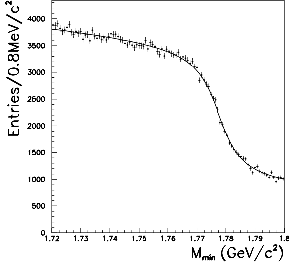
Figure 1: Pseudomass distribution for M_{\min} for the \tau \rightarrow 3\pi\nu candidates. The tau mass is one parameter of the fit shown with a solid line.
