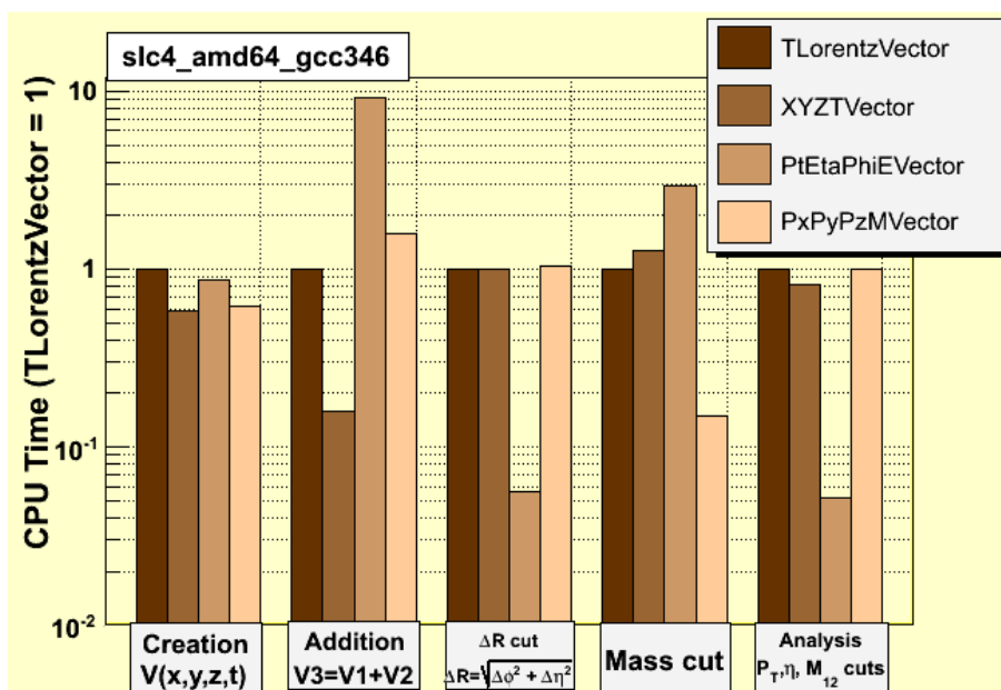
Figure 2: CPU time obtained using TLorentzVector and the new LorentzVector’s based on Cartesian (XYZVector) and on Cylindrical-Eta (PtEtaPhiVector coordinates).
