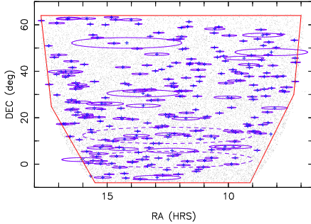
Figure 1: The 270 sources in the CENSORS-Bright sample. The grey area corresponds to the north region of the FIRST survey while the red contour delimits the region of the CENSORS-Bright sample. Each source has S_{1.4\text{GHz}} \geq 1.3\text{Jy} and is represented by a blue cross and circle. The radius of the circle is proportional to the flux of the source, with the exception of the two dashed circles corresponding to 3C 273 ( S_{1.4\text{GHz}}=55\text{Jy} ) and M87 ( S_{1.4\text{GHz}}=142\text{Jy} ).
