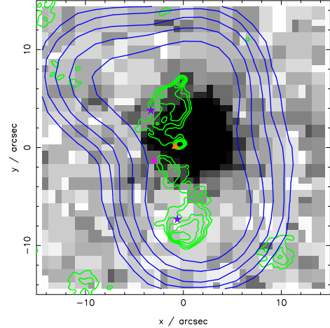
Figure 2: An example of morphology typing. The blue contours are from the FIRST survey, while the green contours are from our new 8GHz VLA observations, which show clearly that the object is FR II in type – the hot spots are at the extremities.
