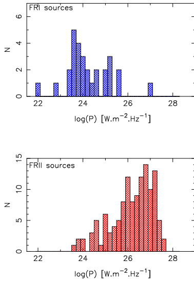
Figure 3: Luminosity distribution by source type. FRI sources are generally less powerful than FRII sources; compact sources (generally quasars) have predominately high luminosities.
