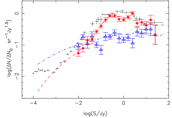
Figure 4: Relative differential source count per \Delta N/\Delta N_0 for all sources (green), FRI (blue) sources, and FRII (red) sources. The NVSS source count is shown as grey crosses for comparison. Here, \Delta N_0 = 1200\Delta(S^{-1.5}) and the error bars correspond to \sqrt{N} where N is the number of object in each bin. The FRII sources dominate the count down to the lower flux densities, where FRI sources take over.
