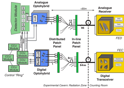
Figure 4: Schematic view of the silicon strip tracker control and readout system. From [8].
