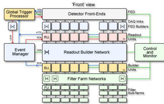
Figure 5: The CMS event builder and related services.
