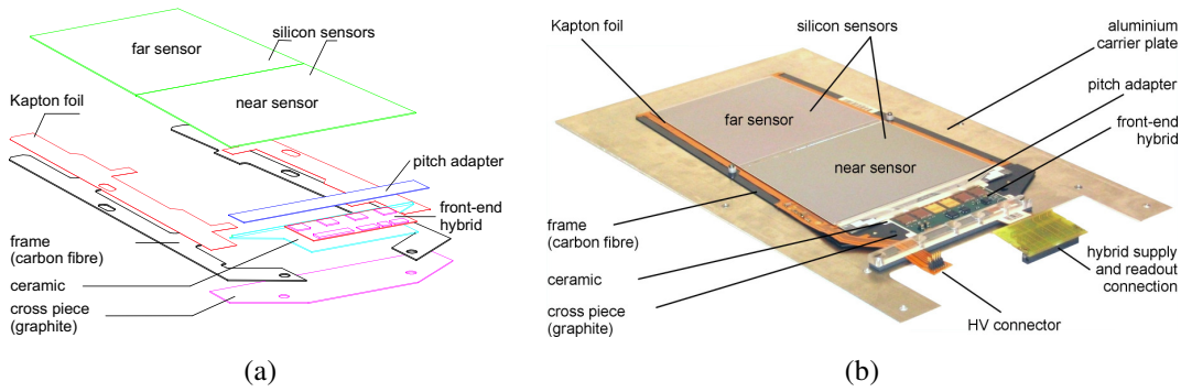
Figure 2: (a) Exploded view of a module housing two sensors; (b) Photograph of a TEC ring 6 module mounted on a carrier plate.
