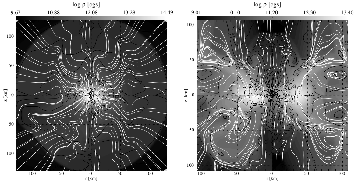
Figure 1: Logarithm of the density (gray-scale) with over-imposed magnetic field lines (white lines) and total magnetic field strength (black contours) corresponding to models collapsing stellar cores with a small initial rotational energy and rotating almost rigidly (left) and with a larger initial rotational energy and differentially rotating (right). Each panel displays the state of the stellar core after the bounce for four different initial magnetic field strengths ( B_0 = 10^{10} G, 10^{11} G, 10^{12} G and 10^{13} G in the clockwise direction starting from the upper left corner). The figures correspond to models of Obergaulinger et al.[41].
