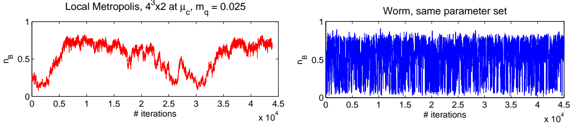
Figure 3: Monte Carlo history of baryon density, for local Metropolis ( left ) and Metropolis+global worm updates ( right ), for runs with m = 0.025, 4^3 \times 2 at \mu_c \approx 0.565 using similar CPU time.
