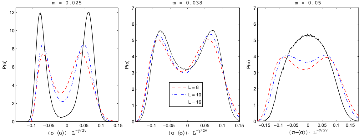
Figure 5: Probability distribution P(\sigma) for masses m = 0.025, 0.038, 0.05 tuned to criticality on systems L^3 \times 2 , L = 8, 10, 16 . A satisfactory data collapse is observed for the middle mass, using Ising critical exponents.
