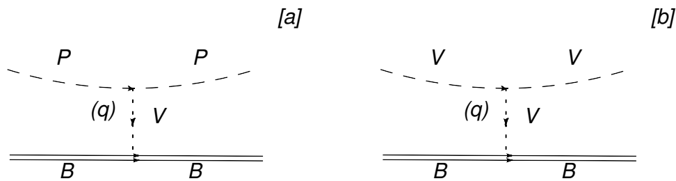
Figure 1: Diagrams obtained in the effective chiral Lagrangians for interaction of pseudoscalar [a] or vector [b] mesons with the octet or decuplet of baryons.
