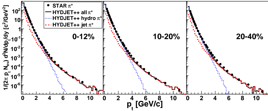
Figure 3: The transverse momentum distribution of positively charged pions in Au+Au collisions at \sqrt{s} = 200A GeV for three centrality sets. The points are STAR data [25], histograms are the HYDJET++ calculations (solid – total, dotted – hydro part, dashed – jet part).
