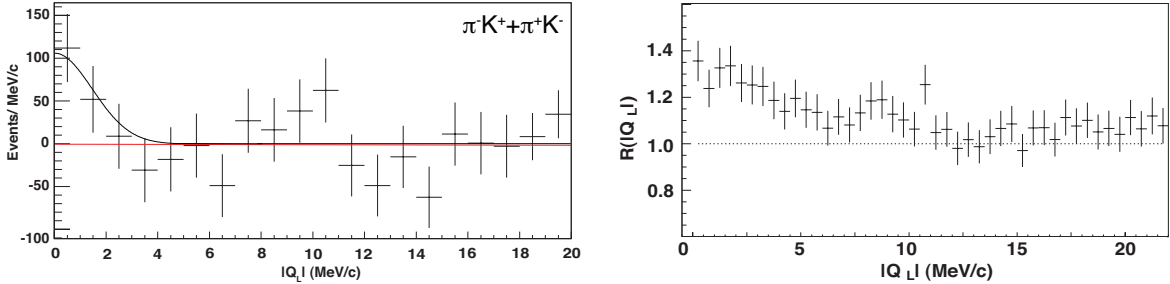
Figure 2: Left: residuals between data and the fitted background for \pi^- K^+ and \pi^+ K^- . A Gaussian fit has been applied (solid line) to illustrate the distribution of atomic-pairs. Right: correlation function R as a function of |Q_L| for \pi K -pairs. The deviation from the horizontal dotted line proves the existence of \pi K Coulomb-pairs.
