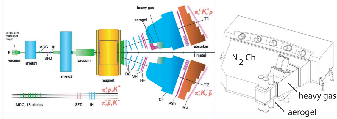
Figure 1: Sketch of the updated DIRAC-II spectrometer, showing the locations of the Čerenkov counters to identify electrons, pions and kaons. MDC = microdrift chambers, SFD = scintillator fibre detector, IH = ionization hodoscope, DC = drift chambers, VH, HH = vertical and horizontal scintillation hodoscopes, PSh = preshower, Mu = muon counters. Right: N_2 , aerogel and heavy gas Čerenkov counters.
