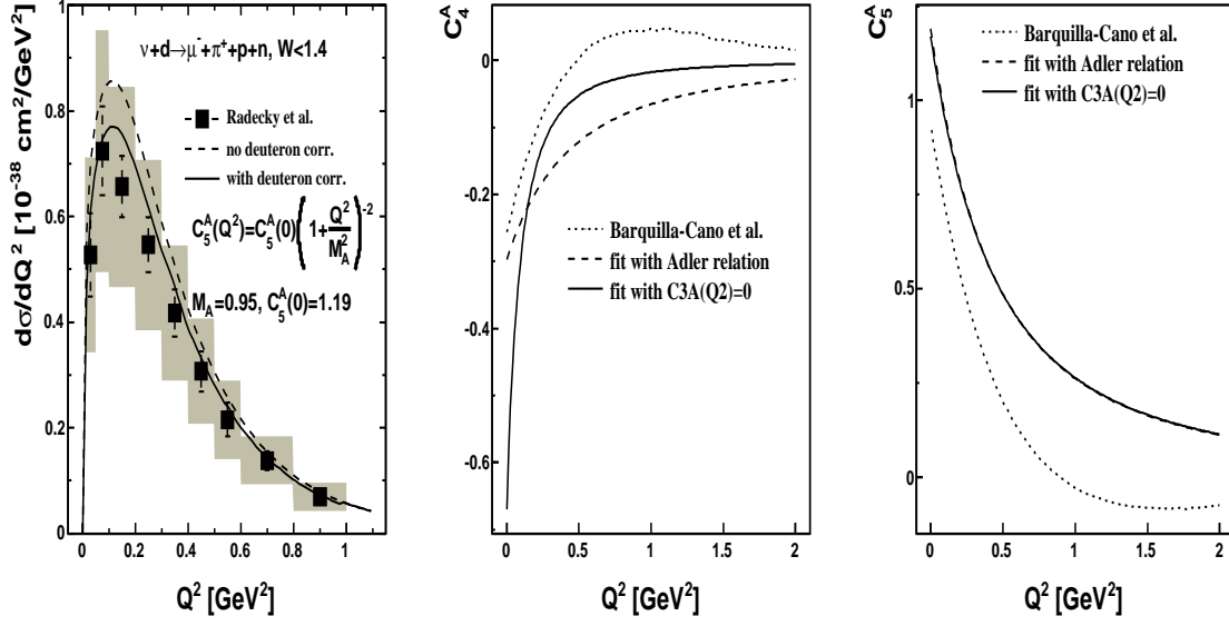
Figure 1: In the first figure the d\sigma/dQ^2 cross sections computed for the ANL beam are plotted (data were taken from [7]). The solid/dashed lines denote the cross sections reduced/not reduced by the deuteron correction. In the second and third figure the C_4^A and C_5^A form factors are plotted. The fits (3.2) are denoted by solid lines. The fits (2.2), computed with C_4^A = -C_5^A/4 , are plotted with dashed lines. The quark model predictions from Ref. [11] are plotted with dotted lines.
