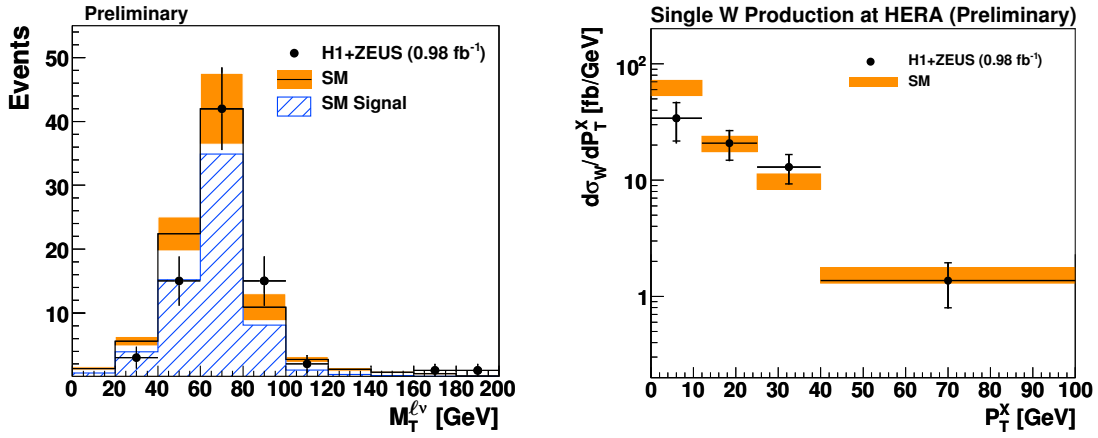
Figure 2: Left: The lepton–neutrino transverse mass M_T^{\ell\nu} of events with an isolated electron or muon and missing transverse momentum. The data (points) are compared to the SM expectation (open histogram). The signal component of the SM expectation, dominated by single W production, is shown as the striped histogram. The total uncertainty on the SM expectation is shown as the shaded band. Right: The single W production cross section as a function of the hadronic transverse momentum, P_T^X . The inner error bar represents the statistical error and the outer error bar indicates the statistical and systematic uncertainties added in quadrature. The shaded band represents the uncertainty on the SM prediction.
