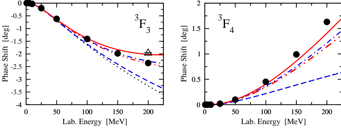
Figure 3: {}^3F_3 - and {}^3F_4 -wave NN phase shifts. The dotted curve is the LO prediction (i.e. based on the pure one-pion-exchange potential). Dashed double-dotted (dashed) and solid (dashed-dotted) lines show the NLO and N^2 LO results with (without) the explicit \Delta -contributions. The filled circles (open triangles) depict the results from the Nijmegen multi-energy PWA [6, 7] (Virginia Tech single-energy PWA [8])
