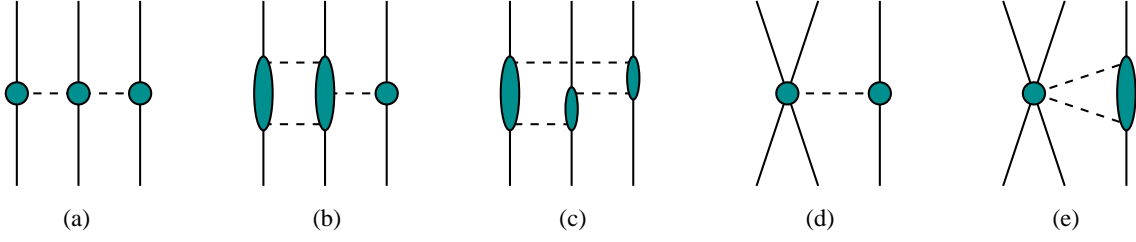
Figure 1: Various topologies that appear in the three-nucleon force at N^3\text{LO} . Solid and dashed lines represent nucleons and pions, respectively. Shaded blobs are the corresponding amplitudes. The long-range part of the three-nucleon force considered in this paper consists of (a) 2\pi exchange graphs, (b) 2\pi - 1\pi diagrams and the ring diagrams (c). The topologies (d) and (e) involve four-nucleon contact operators and are of shorter range.
