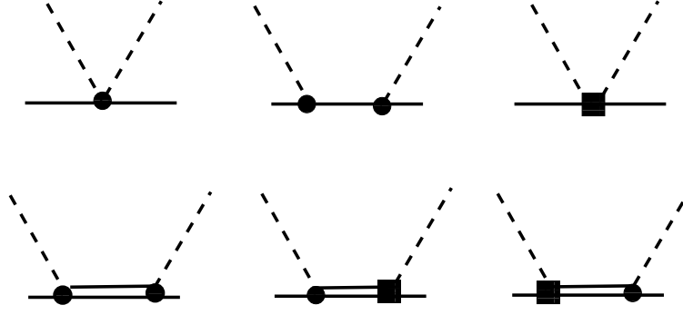
Figure 2: Tree graphs for pion-nucleon scattering at NLO. The filled circles/squares denote leading/subleading vertices. Crossed graphs are not shown.
