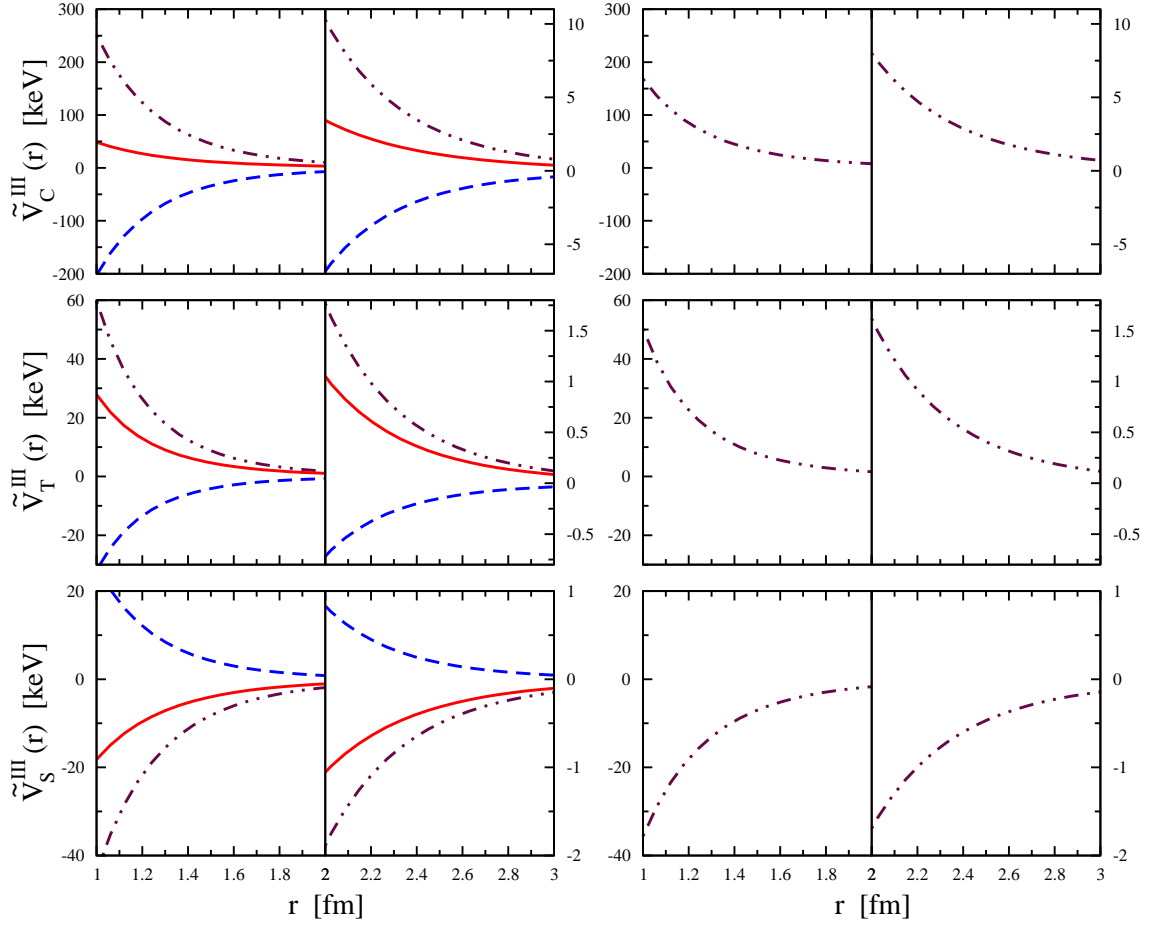
Figure 4: Class-III (CSB) two-pion exchange potential. The left (right) panel shows the results obtained at leading order in chiral EFT with explicit \Delta resonances (at subleading order in chiral EFT without explicit \Delta degrees of freedom). The dashed and dashed-double-dotted lines depict the contributions due to the \Delta - and nucleon-mass differences \delta m_{\Delta}^1 and \delta m_N , respectively, while the solid lines give the total result.
