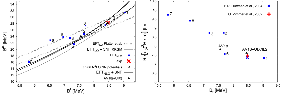
Figure 1: (left) Correlation between the triton and {}^4\text{He} binding energies (Tjon line). The squares are results from the nine NLO \text{EFT}_{\pi} NN potentials. The solid (gray) black lines represent a smooth variation of A_{3NF} for a specific (LO) NLO potential. The upper (lower) dashed line was calculated at LO in [8] with LECs fitted to a_{s,t} ( B(d) , a_s ). The values for AV18(+UIX) are reported in [10], and those using a chiral expansion to NLO and \text{N}^2\text{LO} in [9].
