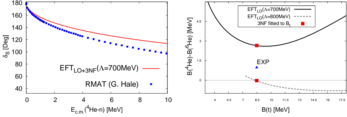
Figure 2: (left) S-wave phase shift in the \frac{1}{2}^+ -channel for ^4\text{He} -n scattering. Compared are the results from a LO EFT _{\neq} calculation (red, solid line) to an R-matrix analysis (blue squares, [13]).
