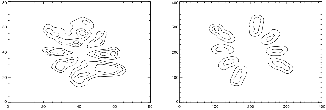
Figure 2: IsovLOCITY contour plots of M33 (left) and the SPH galaxy (right). The four contours are from different channel maps of the HI data cube, with the top contour showing the most blueshifted HI and progressing to the most redshifted HI in the bottom contours. Axes reflect the datacube pixel scales.
