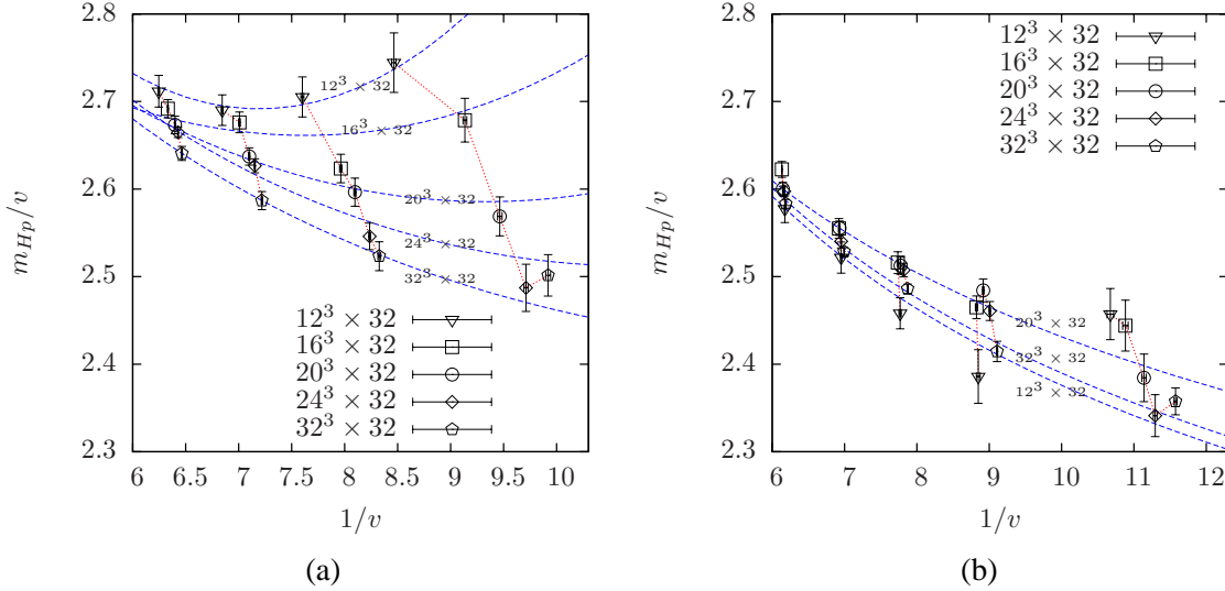
Figure 2: The Higgs propagator mass m_{Hp} is presented in units of the vacuum expectation value v versus 1/v . Those Monte-Carlo results with identical parameter sets differing only in the underlying lattice volume are connected via dotted lines to illustrate the effects of the finite volume. The dashed curves depict the fits of the lattice results according to the finite size fit approach in Eq. (3.9) as explained in the main text. Panel (a) refers to the full Higgs-Yukawa model, while panel (b) shows the corresponding results of the pure \Phi^4 -theory.
