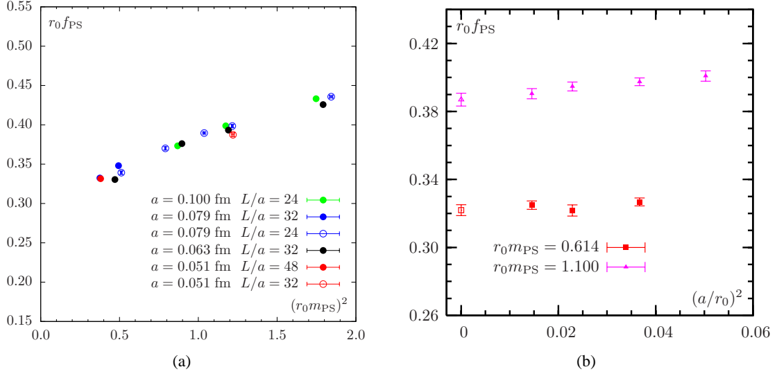
Figure 1: (a) r_0 f_{PS} as a function of (r_0 m_{PS})^2 . (b) Continuum limit scaling: r_0 f_{PS} as a function of (a/r_0)^2 at two fixed values of r_0 m_{PS} and at fixed volume.
