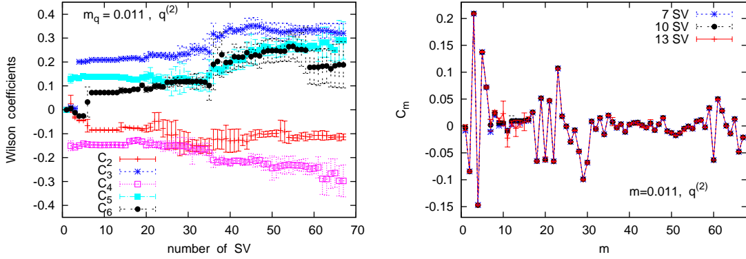
Figure 3: Results for the Wilson coefficients at m_q = 0.011 and q^{(2)} as a varying number of SV is included. Left: the coefficients to the 1-derivative operators for n = 1 \dots 67 reveal a single plateau for n = 7 \dots 13 . Right: the full set C_1 \dots C_{67} agrees very well for n = 7, 10 and 13 , confirming this plateau generally.
