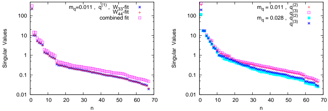
Figure 1: Examples for the rapidly dropping magnitudes of the SV. Due to reflection and rotation symmetries some Wilson coefficients coincide theoretically, e.g. the coefficients of \mathcal{O}_{i,33} in W_{33} , and of \mathcal{O}_{i,44} in W_{44} . We determine the corresponding SV separately, and by a combined fit, which implements this identity. Left: separate and combined SV for m_q = 0.011 , q^{(1)} . Right: combined SV for both quark masses and q^{(2)} , q^{(3)} .
