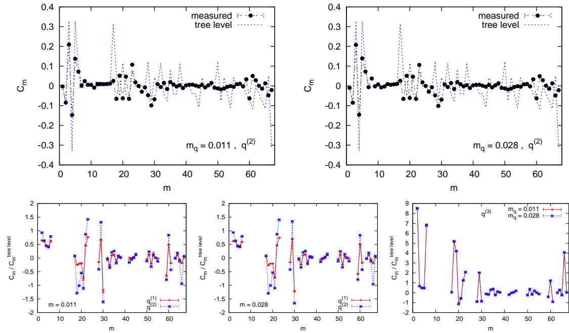
Figure 5: Above: measured Wilson coefficients compared to their tree level values for q^{(2)} . Coefficients for operators with an even number of derivatives take consistently small values. Below: the ratios C_m/C_m^{\text{tree level}} (for non-vanishing denominators). They depend only mildly on the quark mass.
