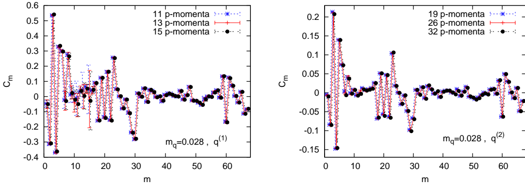
Figure 4: The Wilson coefficients determined from a varying number of the quark momenta. We show results for m_q = 0.028 , at q^{(1)} with 11, 13 or 15 p -momenta (left) and at q^{(2)} with 19, 26 or 32 p -momenta (right). This hardly changes the results for the Wilson coefficients, hence their convergence appears safe.
