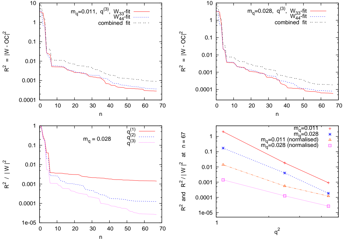
Figure 2: Squared residues R^2 for the operator \bar{\psi}\vec{\gamma}\vec{D}\psi (as an example) against the number n of conditions (corresponding to the SV). The plots above show results of separate and combined fits (as in Fig. 1), for q^{(3)} and m_q = 0.011 (left), and m_q = 0.028 (right). The plot below on the left shows the normalised R^2 for combined fits at m = 0.028 . The final plateau value (at n = 67 ) is compared in the plot below on the right: its decrease for increasing q^2 is roughly linear, so that the relative error remains approximately constant.
