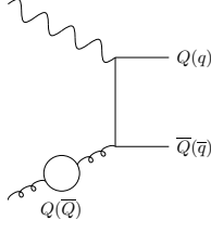
Figure 1: O(a_s^2) virtual heavy quark corrections to H_{g,(2,L)}^{(2)} .
