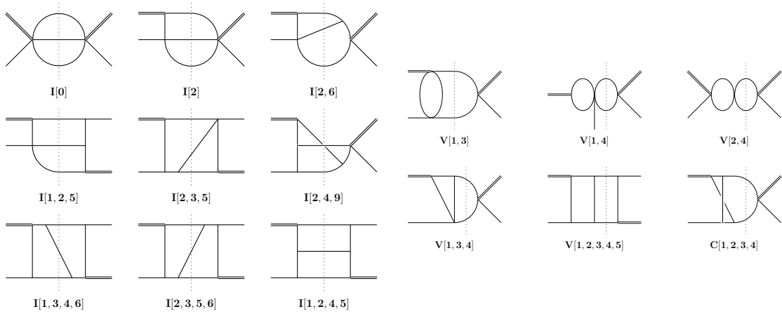
Figure 1: Master integrals for the phase space integration of the double real tree level initial-final antennae at NNLO (left), and for the loop plus phase space integration of the one loop initial-final antennae at NNLO (right). The double line in the external states represents the off-shell momentum, q with q^2 = -Q^2 , the single one is the incoming parton. All internal lines are massless. The cut propagators are the ones intersected by the dotted line.
