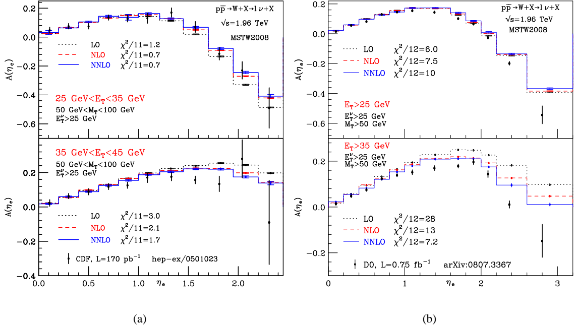
Figure 1: Electron charge asymmetry up to NNLO compared to a) CDF data in the lower E_T region (upper panel) and higher E_T region (lower panel); b) D0 data in the wide E_T region (upper panel) and (high- E_T ) region.
