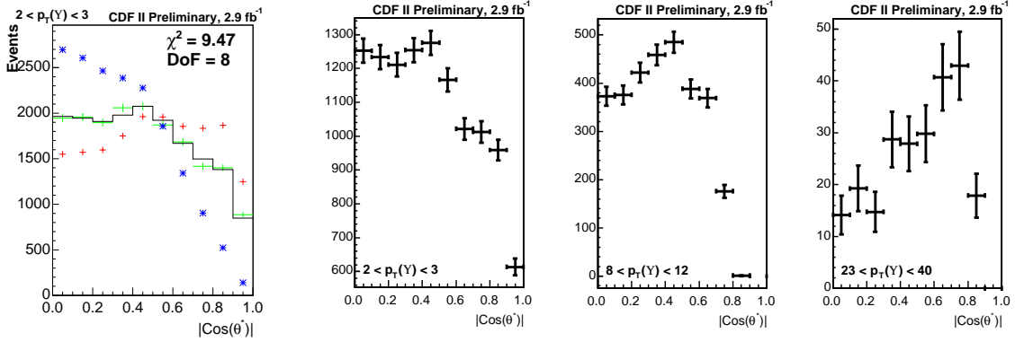
Figure 2: Fit (black) to |\cos \theta^*| distribution (green) for 2 < p_T [\text{GeV}/c] < 3 with T (red) and L (blue) templates (left) and fitted angular distributions of background events for selected p_T bins (right three plots).
