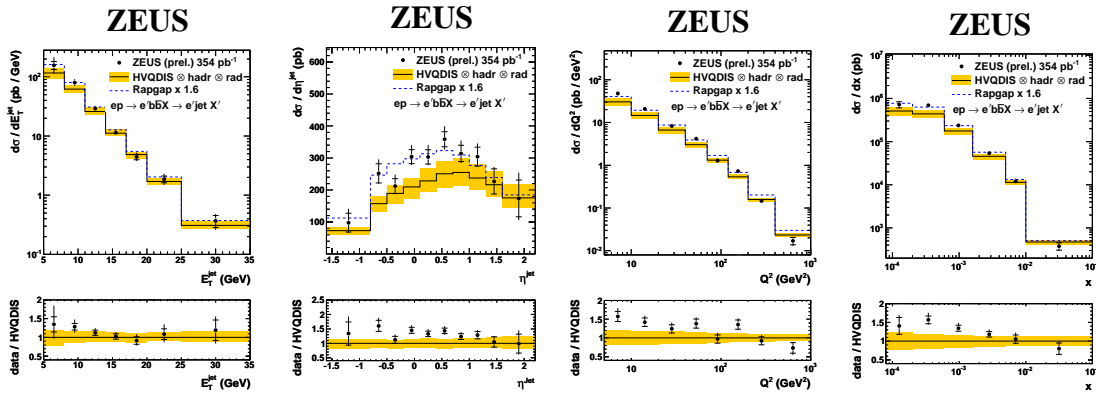
Figure 6: Differential jet cross sections in beauty events as a function of E_T^{\text{jet}} , \eta^{\text{jet}} , Q^2 and x compared to the NLO QCD calculation of HVQDIS and to the RAPGAP MC.
