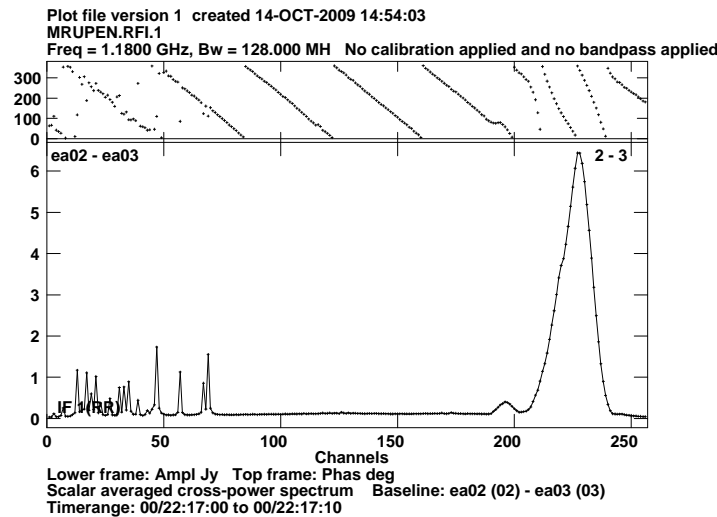
Figure 1: The visibility spectrum for one baseline of the EVLA L-band data
