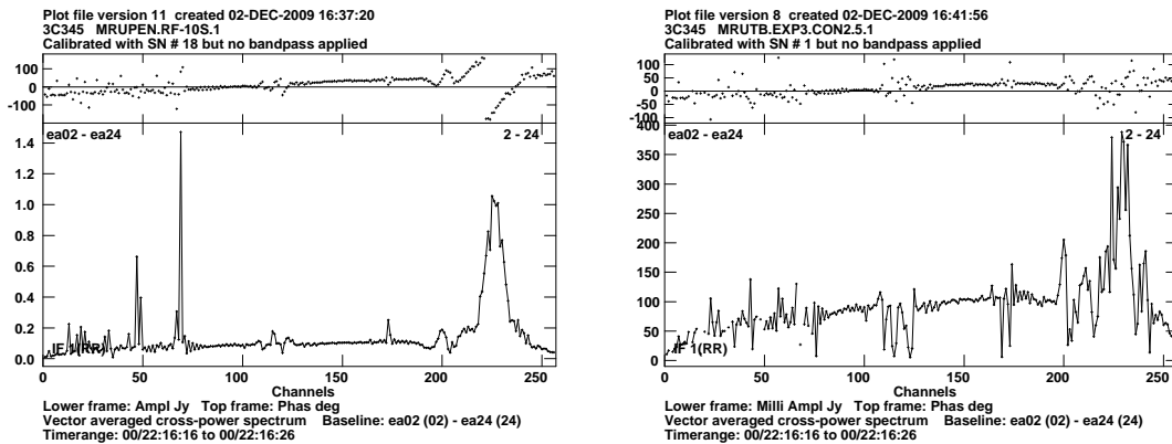
Figure 3: The visibility spectrum for one baseline of the EVLA L-band data. The left plot is the output of the AIPS task UVAVG (vector averaging in 10s). The right plot is the output of UVRFI task. OPTYPE = 'CEXP'. Solution interval = 10s
