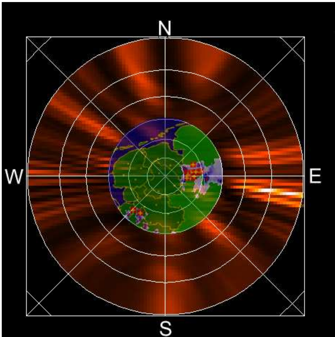
Figure 3: Terrestrial lightning as observed with buenradar (inner part) and LOFAR (outer part).
