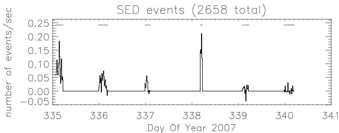
Figure 2: Saturn lightning events observed with UTR-2.
