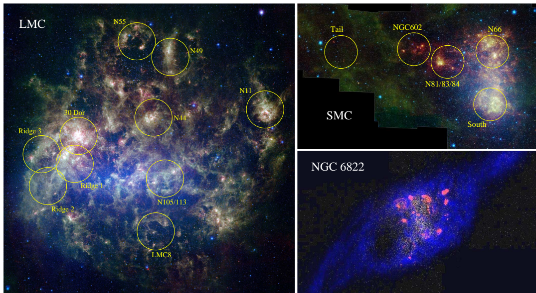
Figure 1: Proposed target fields for MagiKAT — circles are for 1.4-GHz (1°), NGC 682 is covered entirely.
