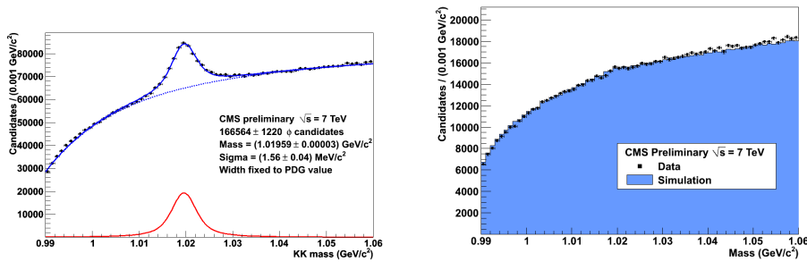
Figure 8: KK invariant mass distributions obtained with the signal-enriched selection (left) and with the anti-K-hypothesis selection (right) using the 7 TeV collision events.
