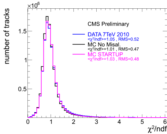
Figure 2: Distribution of the normalized \chi^2 of the reconstructed tracks in \sqrt{s} = 7 TeV collisions compared to simulations with no or realistic misalignment.
