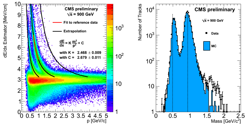
Figure 7: Distribution of the dE/dx estimator vs the track momentum: the black lines represent the expected values for K, protons and deuterons (left); and distribution of the estimated particle mass with the clear contributions of K, protons and deuterons (right) obtained with 900 GeV collision events.
