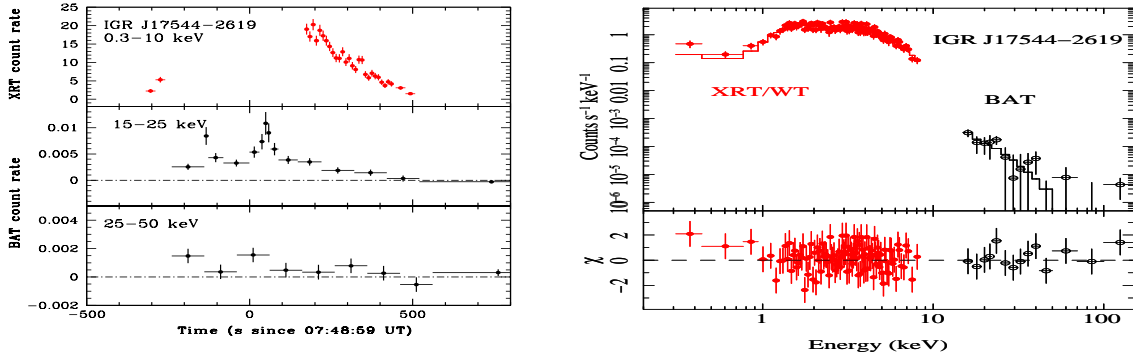
Figure 2: Left: XRT (red) and BAT (black) light curves of the 2009 June 6 outburst of IGR J17544–2619 in units of count s -1 and count s -1 detector -1 , respectively. The XRT data preceding the outburst were collected as a pointed observation, part of our monitoring program. Right: Data from the XRT/WT spectrum and simultaneous BAT spectrum fit with a CUTOFFPL model, and residuals in units of standard deviations.
