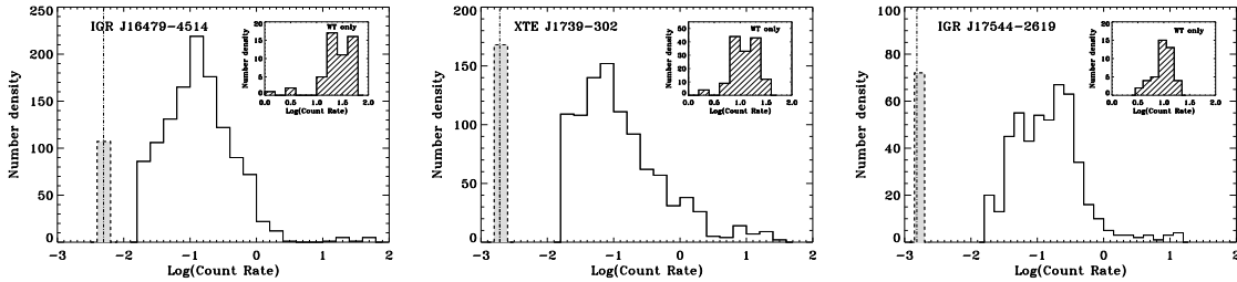
Figure 3: Distribution of the count rates when the XRT light curves are binned at 100 s, for the three sources monitored for two years. The vertical lines correspond to the background. The hashed histograms are points which are consistent with a zero count rate. The insets show the subset of WT data only, binned at 20 s.
