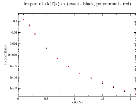
Figure 4: Calculated compared to approximate calculations for the real part of transition matrix element for different energies.
