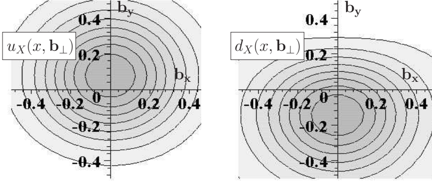
Figure 1: Distribution of the j^+ density for u and d quarks in the \perp plane ( x_{Bj} = 0.3 ) for a proton polarized in the x direction in the model from Ref. [2]. For other values of x the distortion looks similar. The signs of the distortion are determined by the signs of the contribution from each quark flavor to the proton anomalous magnetic moment.
