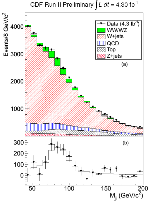
Figure 1: Dijet invariant mass distribution of reconstructed W/Z \rightarrow jj candidates compared to the fitted signal and background components.
