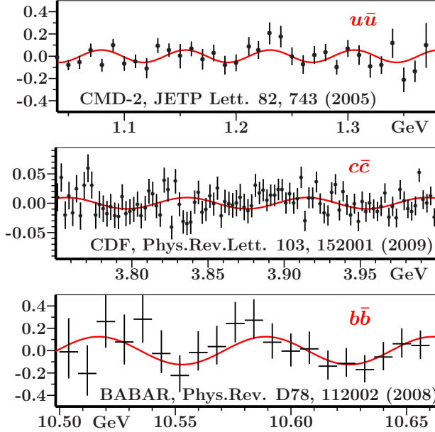
Figure 2: A flavor-independent interference effect is observed by us in data corresponding to e^+e^- (top and bottom) and p\bar{p} (middle) annihilation processes for the production of light quarks, c\bar{c} , and b\bar{b} [23].
