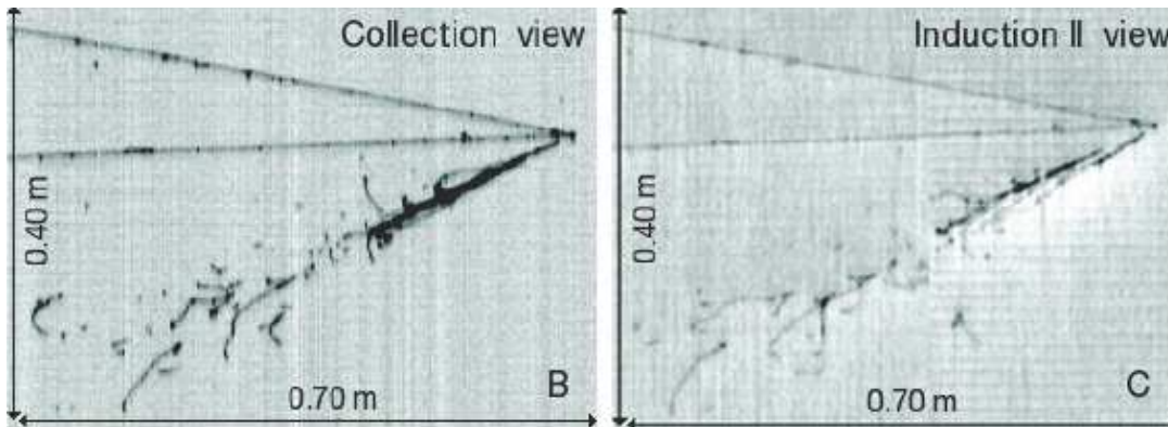
Figure 2: Zoom of the primary vertex region (marked as A in the previous figure) in Collection and Induction II views.
