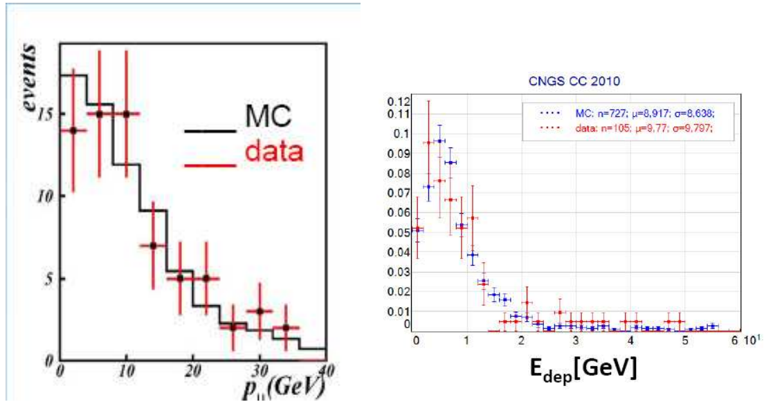
Figure 3: Left: momentum spectrum of muons from \nu_\mu CC interaction reconstructed by multiple scattering, compared with MonteCarlo. Right: distribution of the total deposited energy in \nu_\mu CC interaction events, compared with MonteCarlo.
