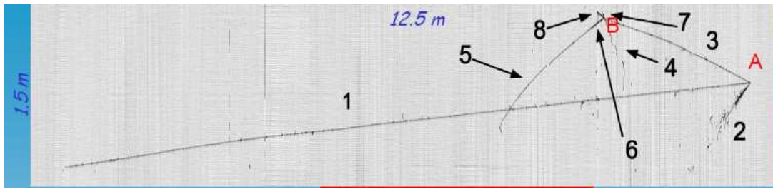
Figure 1: A typical \nu_\mu CC event in ICARUS. The details of vertices and particles are discussed in the text.
