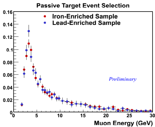
Figure 2 shows the muon momentum distribution for neutrino charged current events that are consistent with starting in the most downstream nuclear target of MINERvA, which has regions of both lead and iron. The distributions have been normalized to equal areas. Table 1 shows the event rates expected in different nuclear targets, assuming 4 \times 10^{20} POT accumulated in the current (Low Energy) Configuration.
