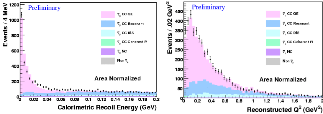
Figure 1 shows (left) the calorimetric recoil energy away from the muon that is located in the charged current event candidates, and (right) the reconstructed Q^2 distribution of the remaining events after a cut on calorimetric energy is made. Both plots are area normalized and only the statistical uncertainties are shown.
