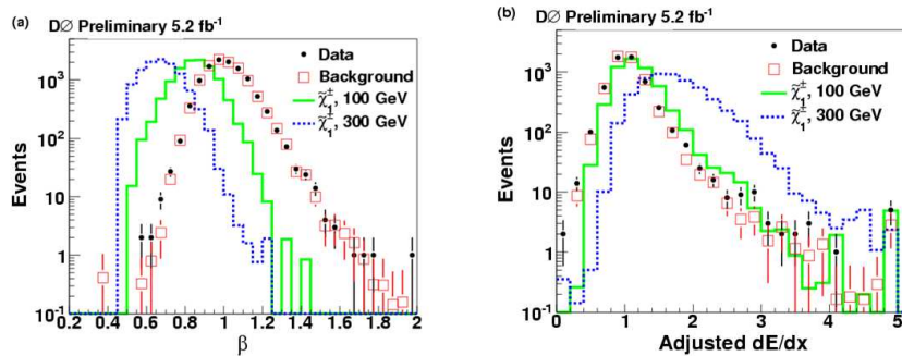
Figure 1: \beta and dE/dx distributions of the highest p_T muon in the event for data, background, and gaugino-like charginos. The distributions are normalised to have the same number of events.
