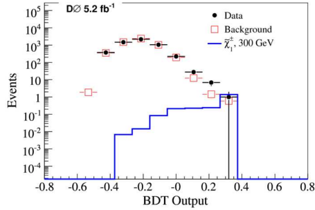
Figure 2: BDT output for data, background, and signal (gaugino-like chargino of mass 300 GeV) are shown.
