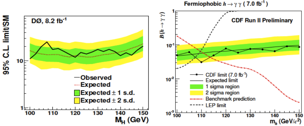
Figure 2: Observed and expected 95% CL upper limits on \sigma \times \text{Br}(H \rightarrow \gamma\gamma) relative to the SM prediction, as a function of the SM Higgs boson mass for D0 (left). Similarly for the fermiophobic Higgs model, the limits on \text{Br}(H \rightarrow \gamma\gamma) are shown for CDF (right). The shaded regions represent the probability of fluctuations of the observed limit away from the expected limit based on the distribution of simulated experimental outcomes under the background-only hypothesis.
