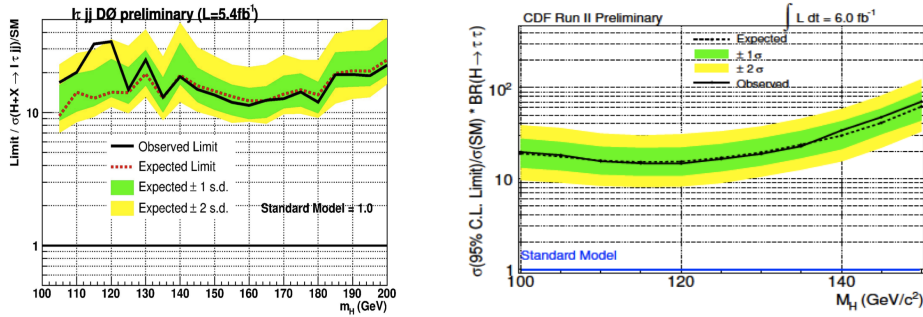
Figure 3: 95% C.L. limit on Higgs boson production rate times branching ratio over the SM expectation as a function of the Higgs boson mass at D0 (left) and CDF (right).
