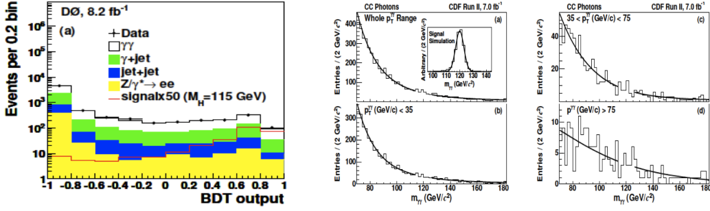
Figure 1: The BDT output distributions for the SM (left). The invariant mass distribution of central-central photon pairs (center and right): (a) the entire p_T^{\gamma\gamma} region used for the SM Higgs boson search and three separate p_T^{\gamma\gamma} regions in (b) p_T^{\gamma\gamma} < 35 GeV, (c) 35 < p_T^{\gamma\gamma} < 75 GeV, and (d) p_T^{\gamma\gamma} > 75 GeV.
