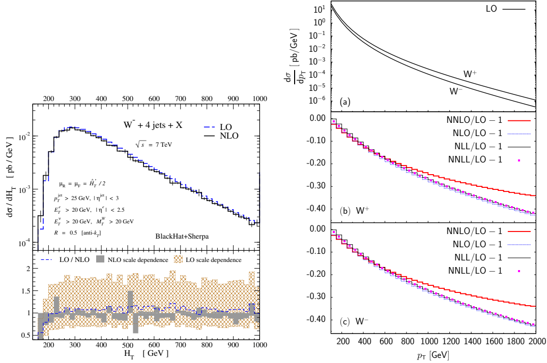
Figure 4: Left: NLO QCD corrections to W^- + 4 \text{ jets} production at the LHC [31]; top: Differential distribution of the transverse energy H_T \equiv \sum_j E_{T,j}^{\text{jet}} + E_T^e + E_T^{\nu} ; bottom: K -factor and scale dependence; note the marked reduction of scale uncertainties at NLO. Right: Relative EW corrections to the p_T distribution for on-shell W^\pm + \text{jet} production at the LHC, and corresponding relative corrections [33]. (NNLO = NLO + 2-loop NLL; NLL and NNLL considered at one loop)
