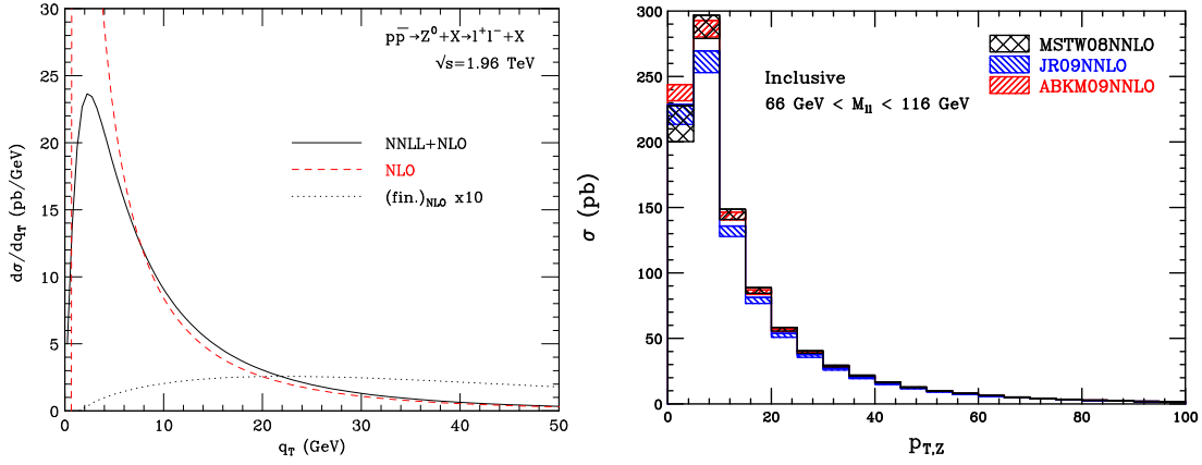
Figure 1: Left: Comparison of the resummed result at NNLL accuracy to the fixed-order computation at the Tevatron [5] for the Drell–Yan process. The fixed-order prediction fails for q_T < 10 \text{ GeV} . ((fin.)_{NLO} : Non-logarithmically-enhanced contributions). Right: Distribution of the Z-boson transverse momentum at NNLO accuracy for different PDF sets at the LHC (FEWZ [8]).
