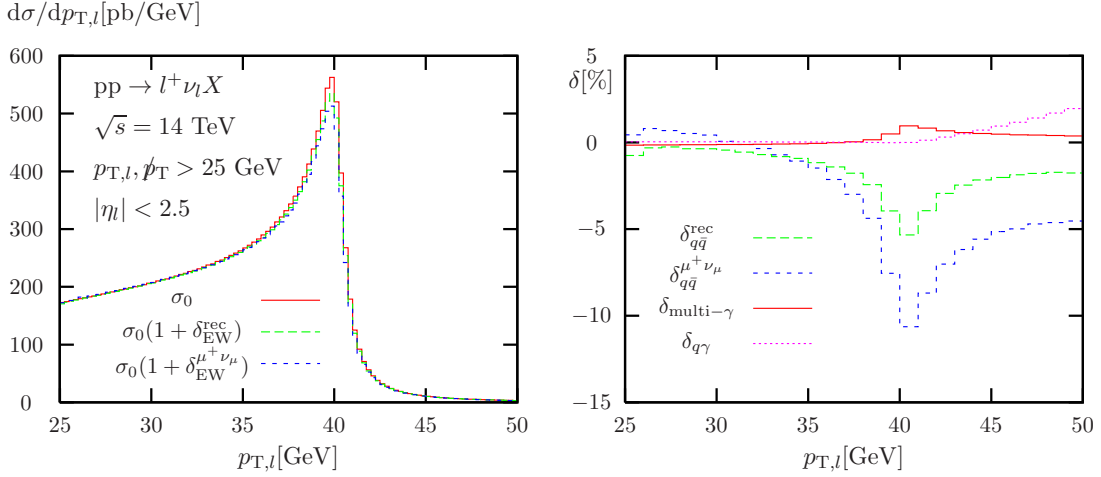
Figure 2: EW corrections to the lepton transverse momentum for the CC Drell–Yan process at the LHC [14]. Results are presented for bare muons ( \delta_{q\bar{q}}^{\mu^+\nu\mu} ) and for electrons employing electron-photon recombination ( \delta_{q\bar{q}}^{rec} ), respectively; the effects due to multi-photon radiation ( \delta_{multi-\gamma} ) as well as photon-induced processes ( \delta_{q\gamma} ) are small.
