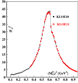
Figure 2: Pion form factor |F_{\pi}|^2 obtained by \pi\pi\gamma/\mu\mu\gamma ratio (KLOE11) and the previous (KLOE10) analysis.
