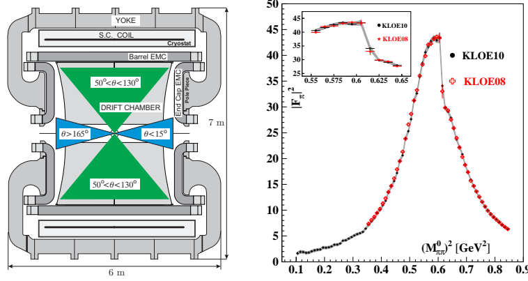
Figure 1: Left: Schematic view of the KLOE detector with selection regions; Right: Pion form factor |F_\pi|^2 obtained in KLOE10 and the previous (KLOE08) analysis.
